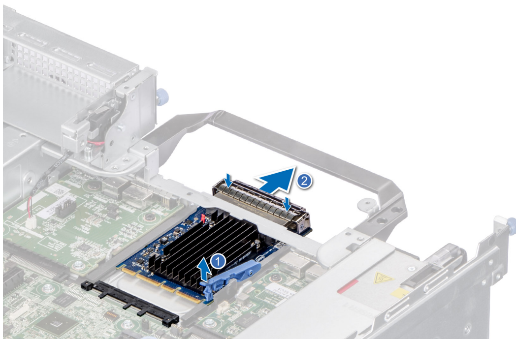
Figure 140. Removing the OCP card
