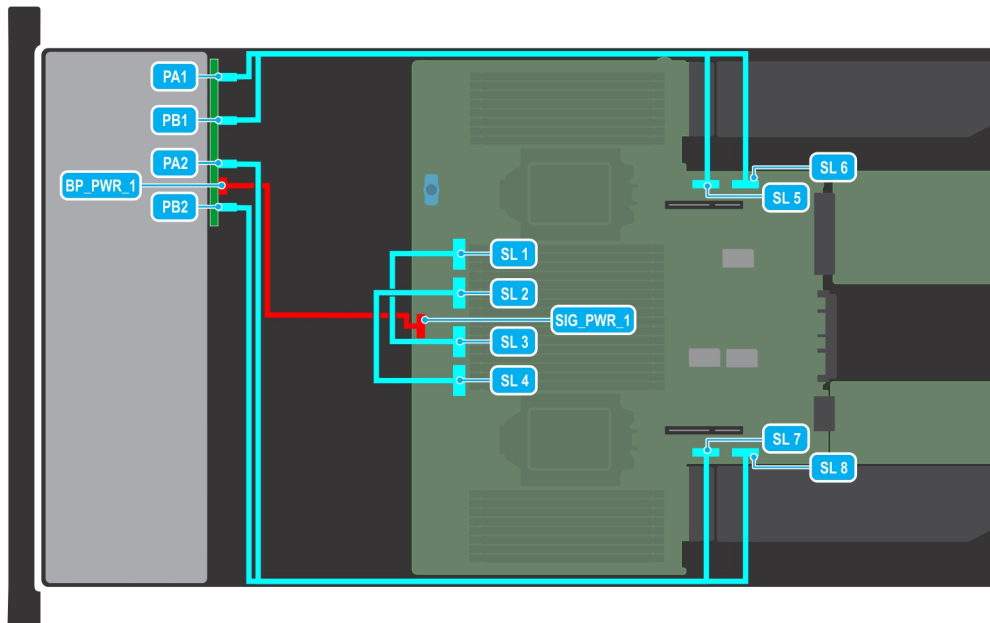
Figure 63. 8 x 2.5-inch with NVMe
